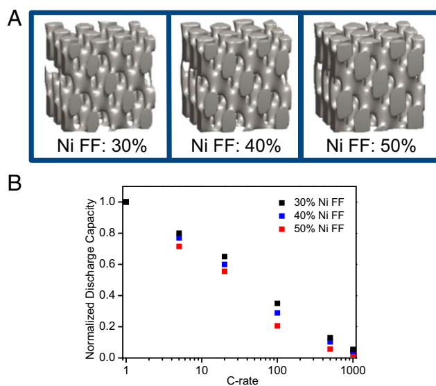
Fig. 5. Influence of electrode porosity on the power performance of 3D microbatteries. (A) Schematics of 3D nickel current collectors with various filling fractions (FFs). (B) Normalized discharge capacity of microbatteries with various nickel FFs at C rates ranging from 1 to 1,000.
